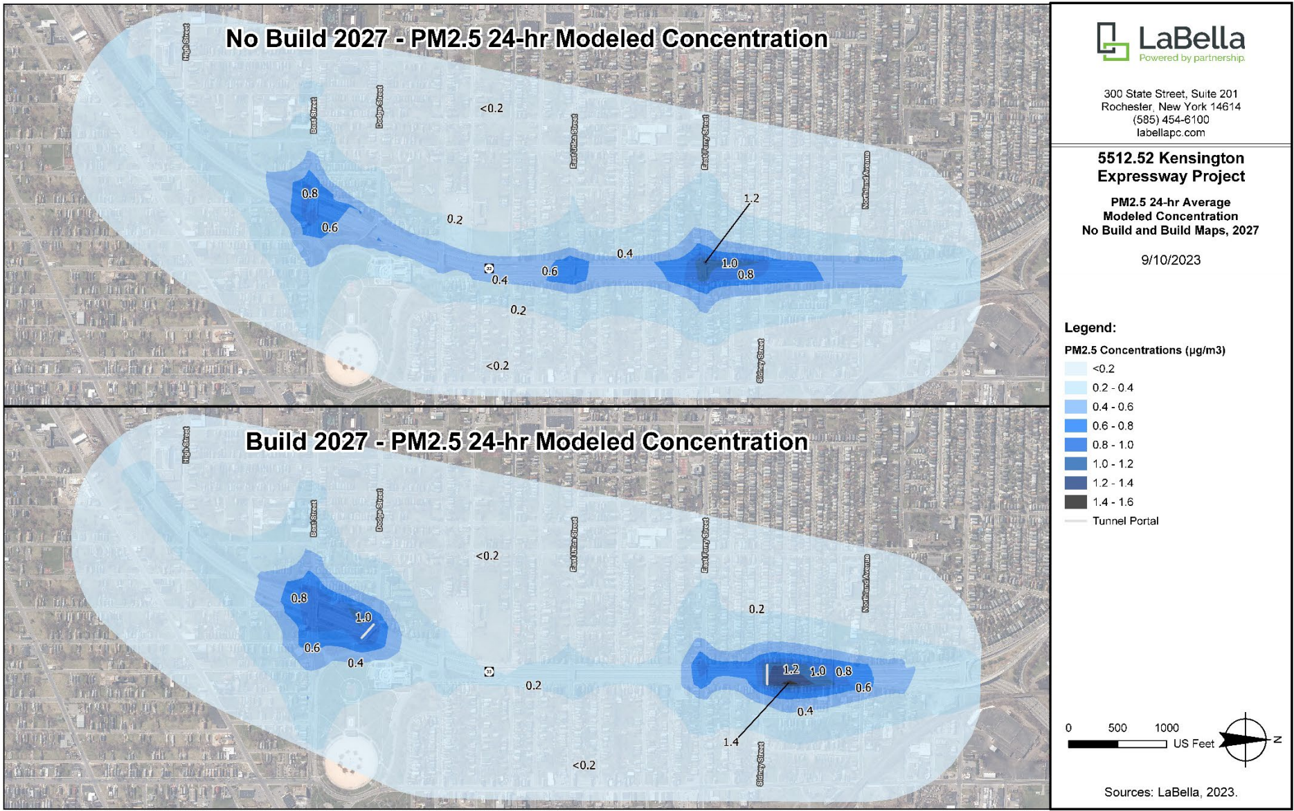
Figure 9: Modeled Year 2027 24-hour Average PM2.5 Concentrations
