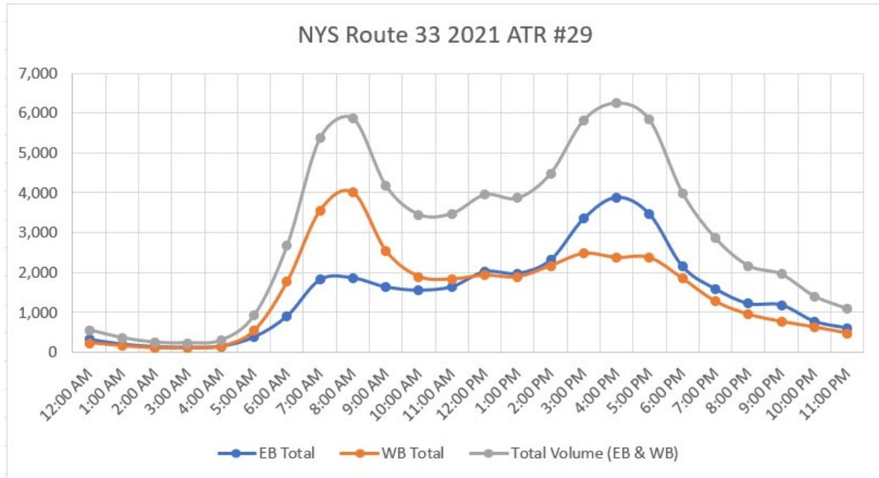
Figure 3: NYS Route 33 Existing 24-hr Traffic Counts
