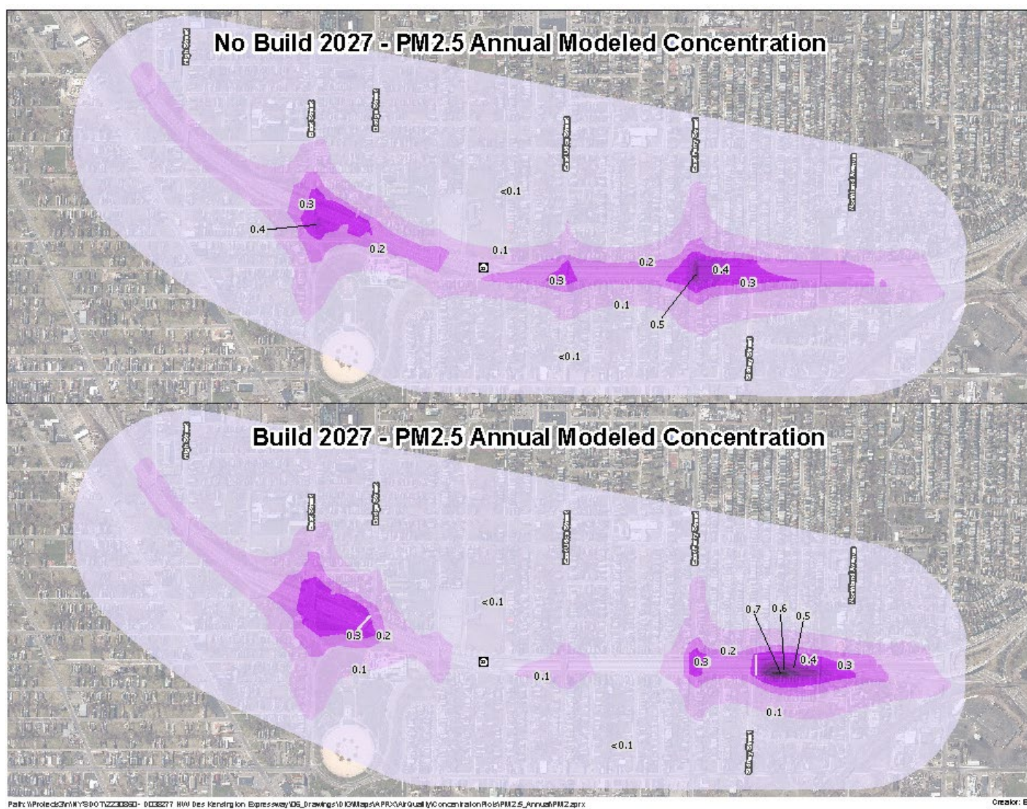
Figure 11 Modeled Year 2027 Annual Average PM2.5 Concentrations
