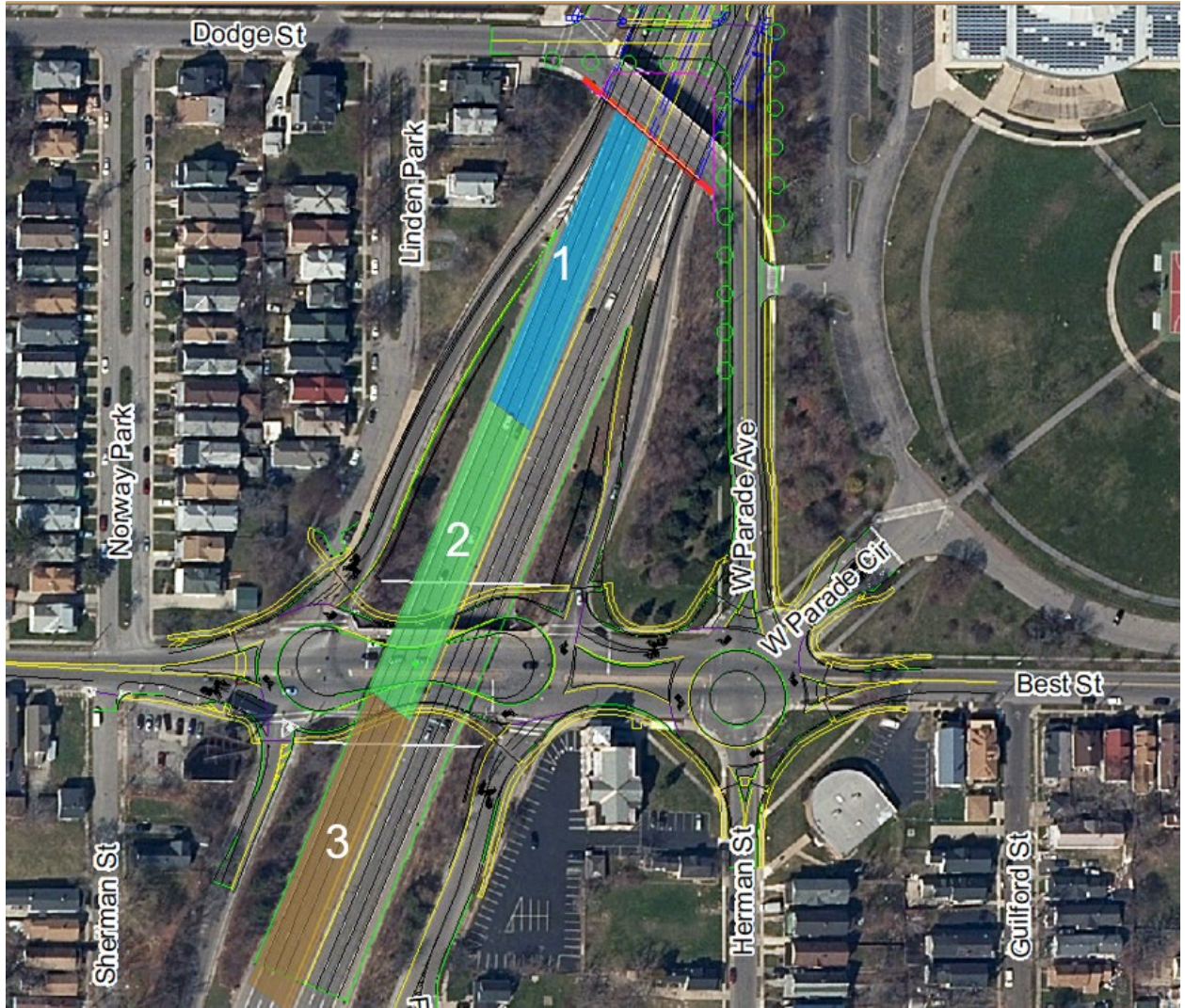
Figure 4: Dodge Street Portal Jet
